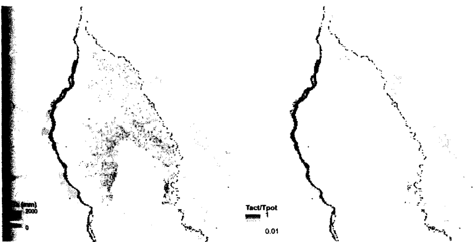
Figure 8.8 (a) Annual actual evapotranspiration ( \text{ETa} ) and (b) ratio of actual to potential transpiration ( \text{Ta Tp}^{-1} ) in the Gezira scheme in 2007
