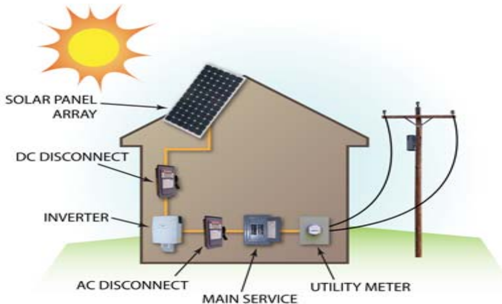
Fig. 1. Typical setup for a grid connected PV system (EnSol Energy Solution Providers, No Date)
