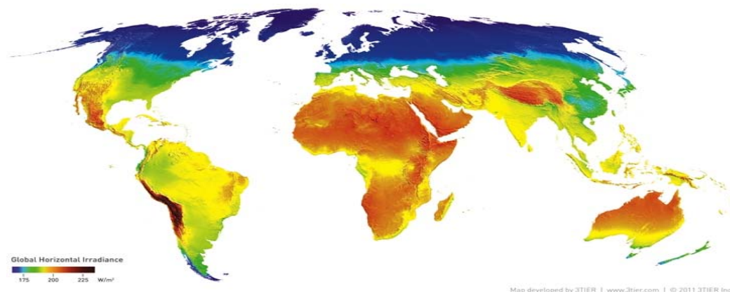
Fig. 4. Solar radiance over the globe (Sustainable Energies, No Date)
