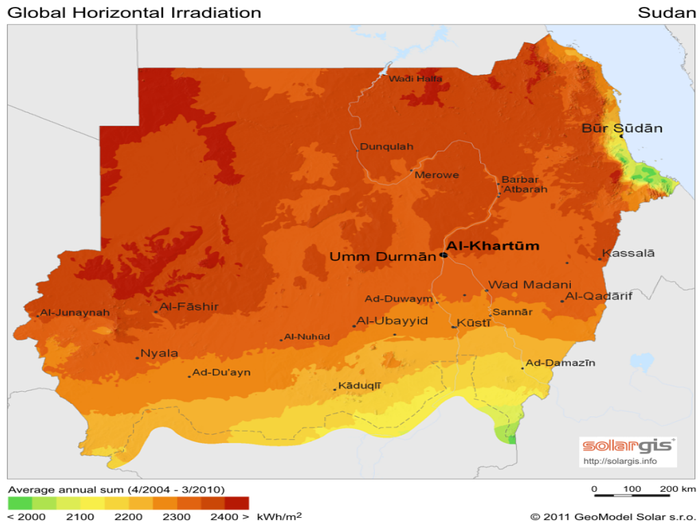
Fig. 5. Sudan's Global Horizontal radiance map (GeoSun Africa, 2017)
